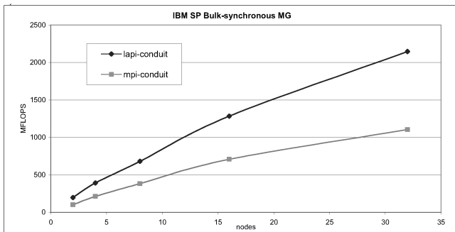
Figure 7 Performance for a bulk-synchronous UPC implementation of NAS multigrid using different network APIs with the Berkeley UPC compiler on an IBM SP
