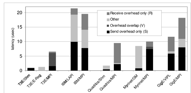
Figure 1 Send and receive software overheads ( o_s and o_r ) superimposed on the one-way end-to-end latency (EEL) for 8-byte messages on various high-performance systems. For MPI on the T3E and Myrinet, the sum of the overheads is greater than EEL, and so o_s = S + V and o_r = R + V . For the other configurations o_s = S and o_r = R
