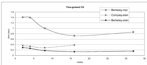
Figure 2 Performance for a naively (fine-grained) UPC implementation of NAS conjugate gradient using different network APIs/compiler on a Compaq AlphaServer
