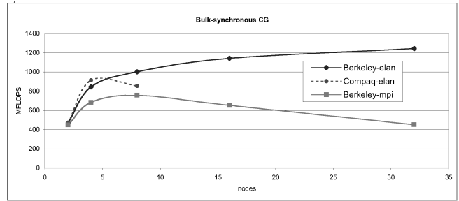
Figure 3 Performance for a bulk-synchronous UPC implementation of NAS Conjugate Gradient using different network APIs/compiler on a Compaq AlphaServer
